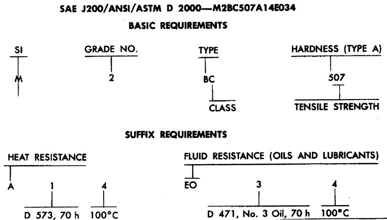
FIGURE 1—LINE CALL-OUT
